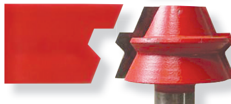
22 1/2° Lock Miter Bit (99-043)
